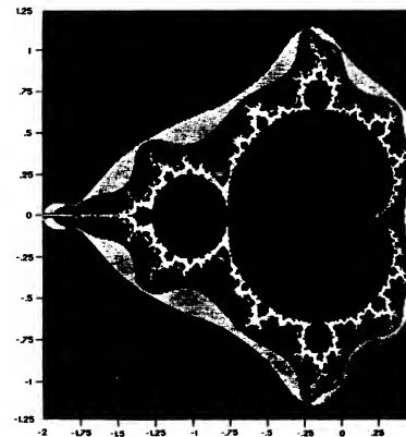
THE MANDELBROT SET
